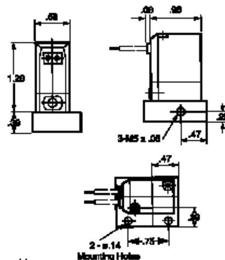
#94 K3P on a subbase
