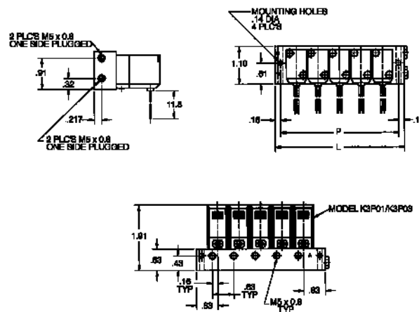
#94A K3P on a subbase
